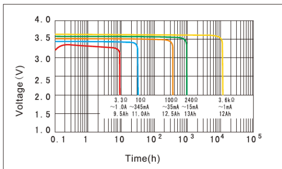
Discharge characteristics at 25°C
