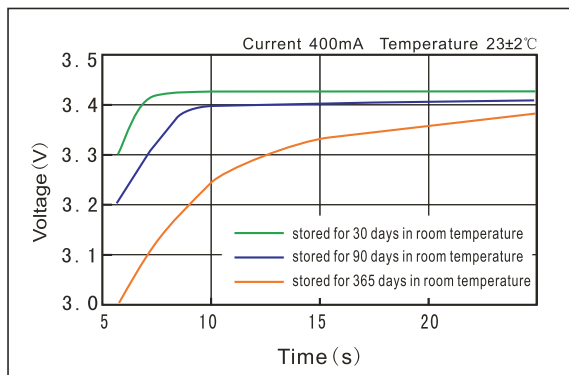
Discharge characteristics after storage
