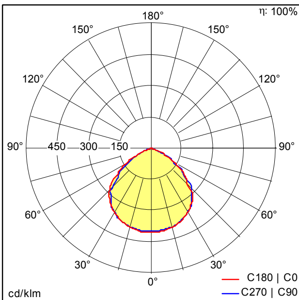
TE_LEONIE_LED_FL_IP65_30W_840.idt
