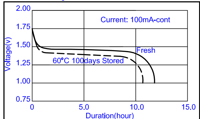
Discharge Characteristics
