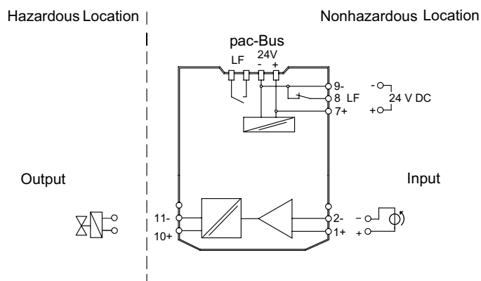
Connection Diagram 9175/10-16-11
