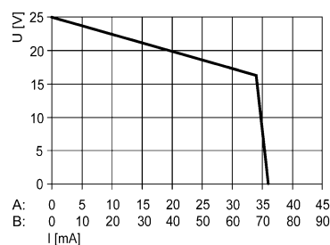
Output characteristic 9175/.0-16-11; 9176/.0-16-00
