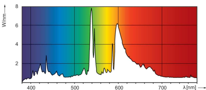
Spectral Power Distribution Colour - MASTERC CDM-Tm Mini 20W/830 PGJ5 1CT/12
