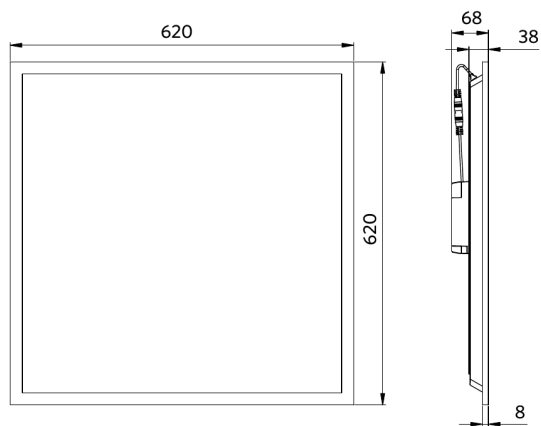
LEDPanelS-E4 Sq620-32W
