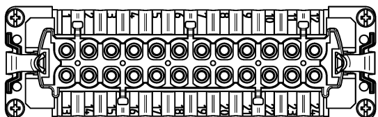
24-polig/24-pole 70.300.2440.0
