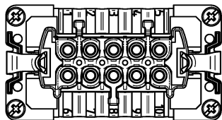
10-polig/10-pole 70.300.1040.0
