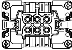
6-polig/6-pole 70.300.0640.0
