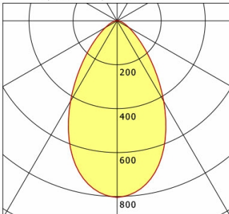
Flixx 300 Square (FLIQZ 300.24, 1xLED 11W 830/3000K 980lm)
