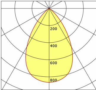
Flixx 300 Square (FLIQZ 300.05, 1xLED 11W 830/3000K 1010lm)
