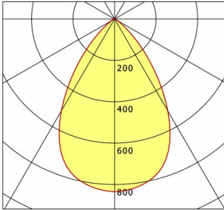
Flixx 300 Square (FLIQZ 300.25, 1xLED 11W 830/3000K 1000lm)
