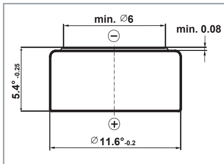
Diameter: 11.60 mm Height: 5.40 mm
