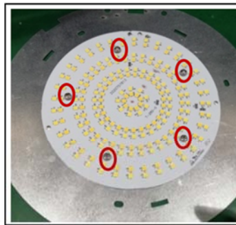
Figure 3 Remove the screws
