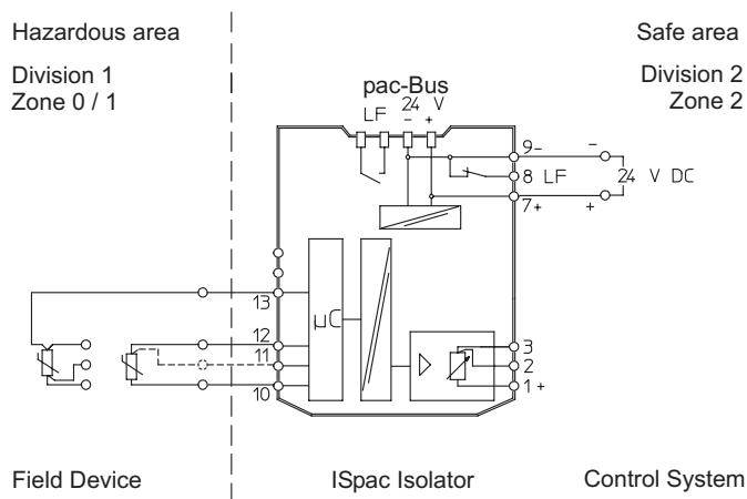
Connection diagram 9180/1.-77-11
