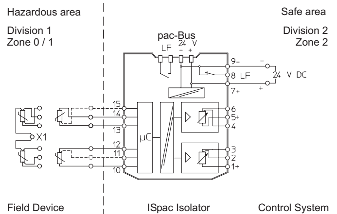
Connection diagram 9180/2.-77-11
