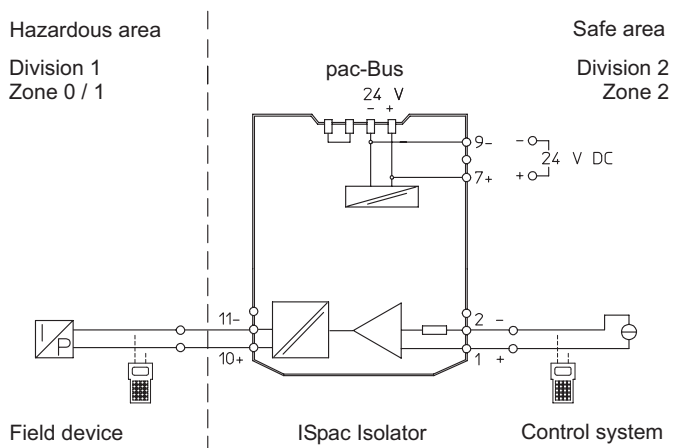
Connection diagram 9165/16-11-10
