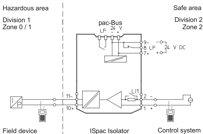
Connection diagram 9165/16-11-11
