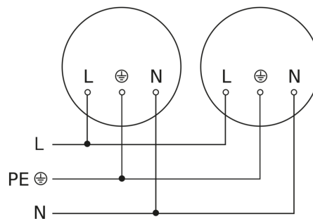
Master/slave interconnection circuit diagram
