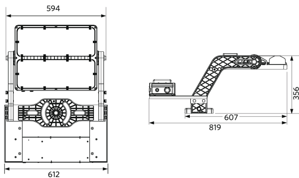
LEDfloodOly-P Re600-600W
