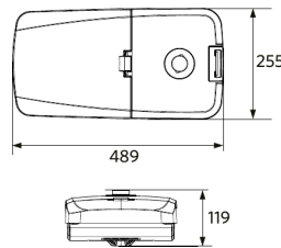
LEDRoad-St-P2 Re489 Zhaga
