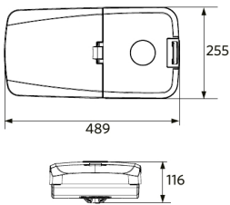
LEDRoad-St-P2 Re489 On-Off & DALI2
