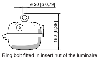
Ring bolt fitted in insert nut of the luminaire
