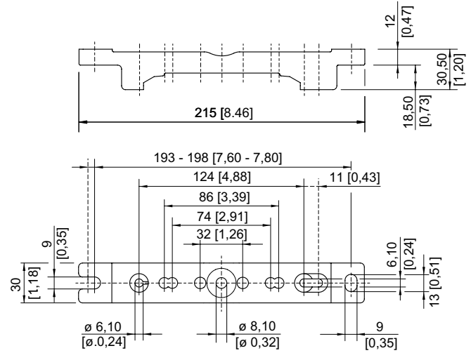
Mounting rail
