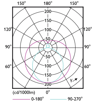
General uniform lighting - MAS LEDtube 1200mm HE 16.5W 840 T5 EU Light Distribution Diagram - MAS LEDtube 1200mm HE 16.5W 840 T5 EU
