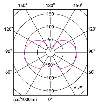
Light Distribution Diagram - MAS LEDBulbDT5.9-60W E27 927A60CL G
