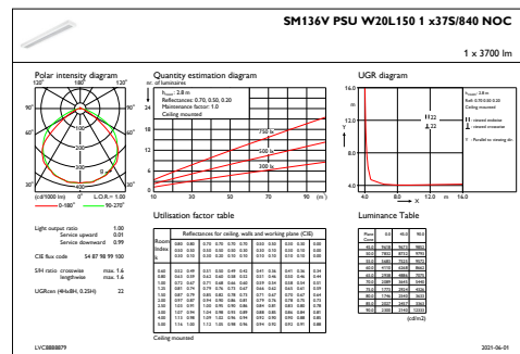
IFGU1_SM136VPSUW20L1501x37S840NOC
