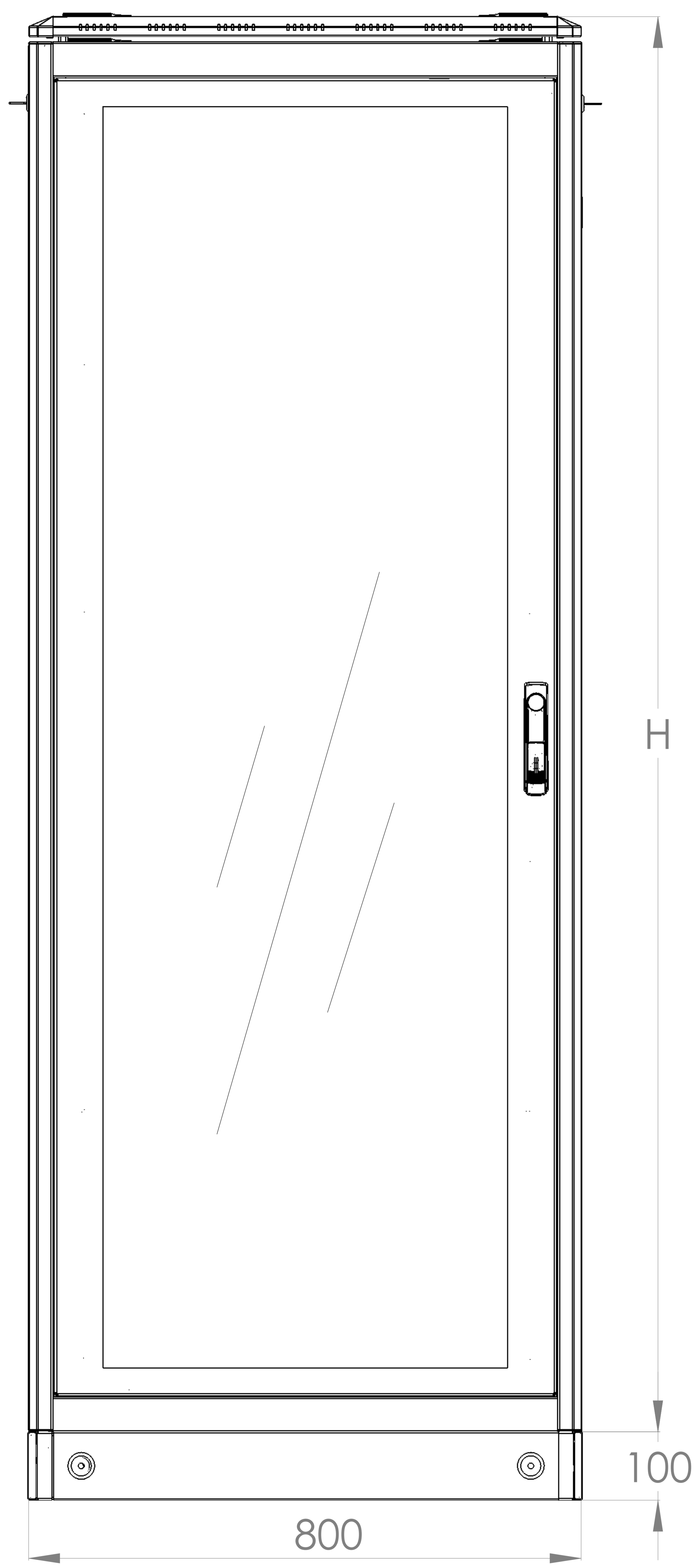
FRONT VIEW
