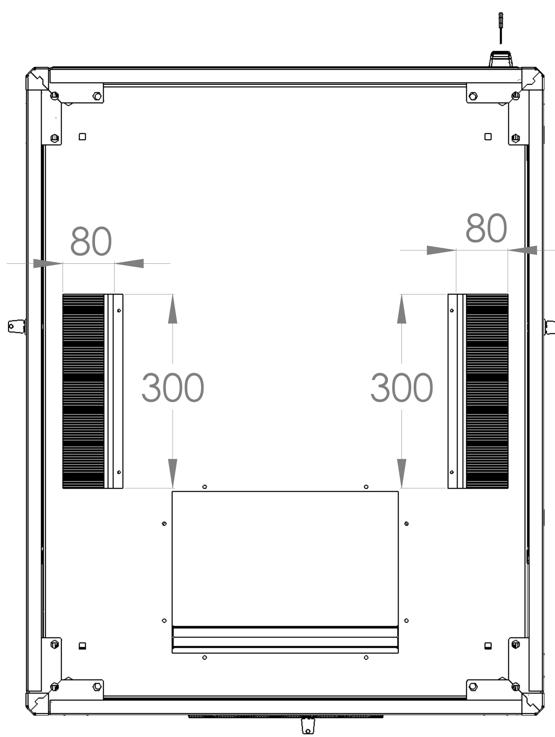
BOTTOM VIEW
