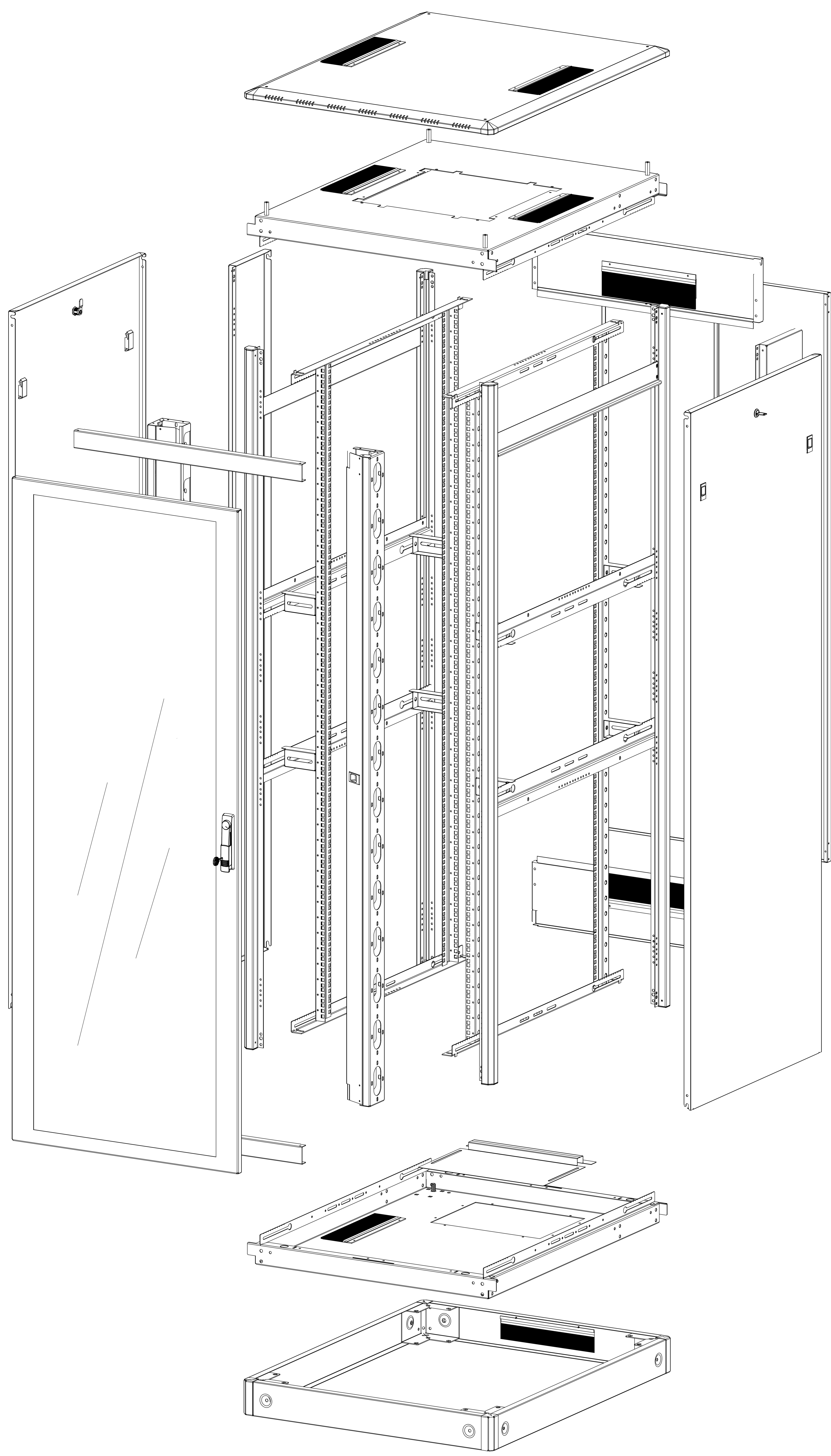
EXPLODED VIEW
