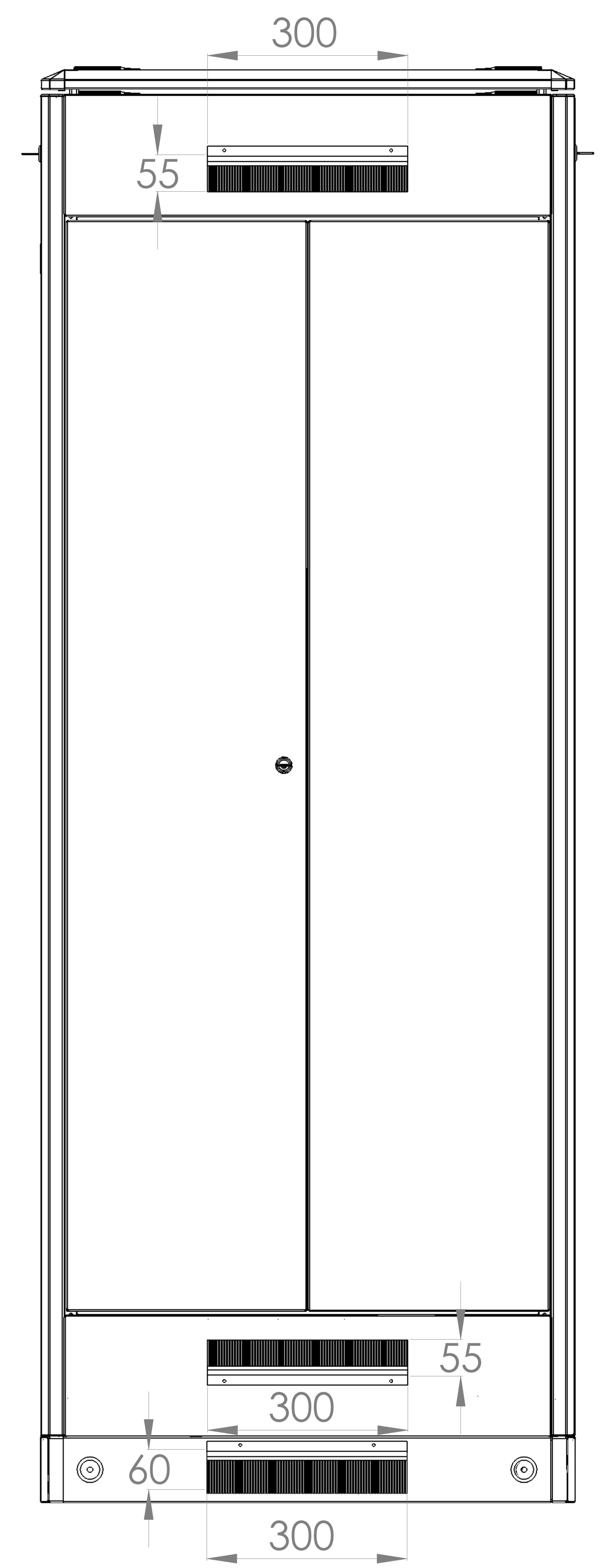
REAR VIEW
